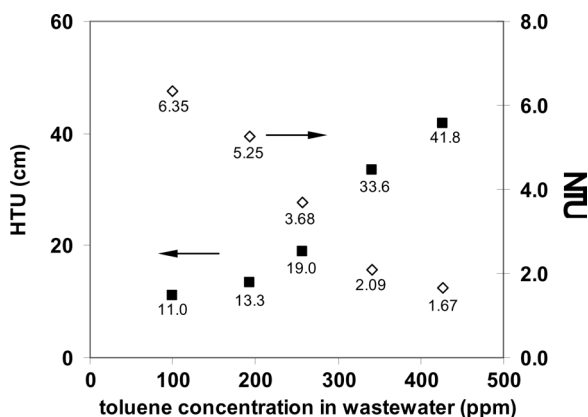
Figure 10. Height of transfer unit (HTU) and number of transfer unit (NTU) as a function of toluene concentration in wastewater feed.
