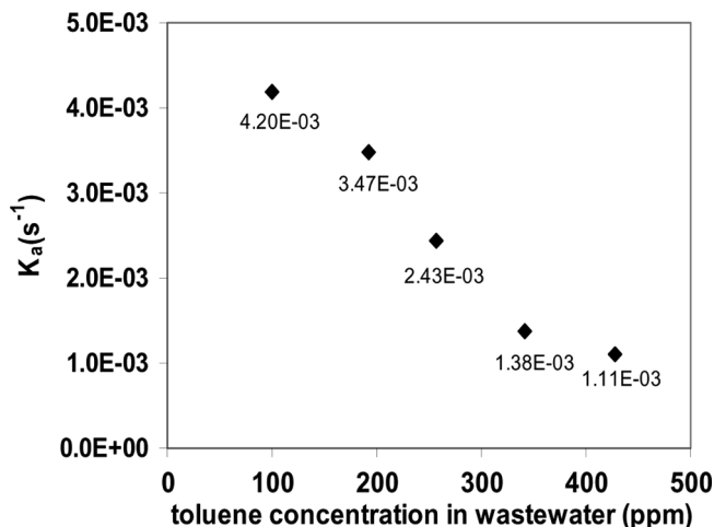
Figure 11. Overall volumetric mass transfer coefficient ( K_a ) as a function of toluene concentration in wastewater feed.
