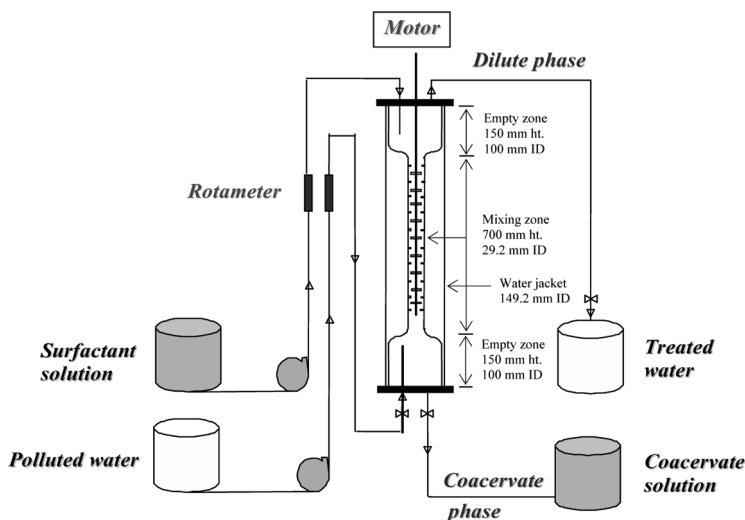
Figure 1. Schematic of the cloud point extraction pilot unit.
