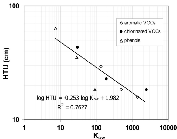
Figure 5. Height of transfer unit (HTU) as a function of octanol-water partition coefficient ( K_{ow} ) of the various solutes in continuous operation.
