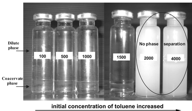
Figure 8. Pictures of phase separation of nonionic surfactant solution at various initial concentrations of toluene (ppm). Condition: 70 mM surfactant in initial solution and 40°C operating temperature.
