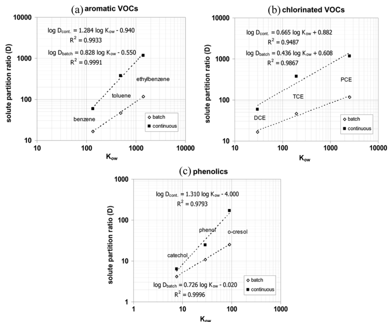
Figure 3. The correlation of solute partition ratios ( D ) and octanol-water partition coefficient ( K_{ow} ) of aromatic VOCs, chlorinated VOCs, and phenolics, respectively in batch and continuous operation.
