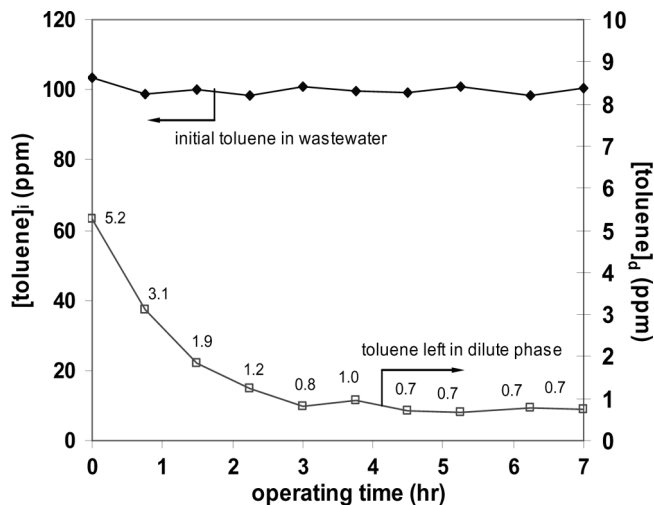
Figure 2. Toluene concentration as a function of operation time. Condition: 350 mM surfactant feed solution, 100 ppm toluene in wastewater, 100 rpm rotating disc speed, 40°C operating temperature and wastewater/surfactant solution flowrate ratio 12.65.
