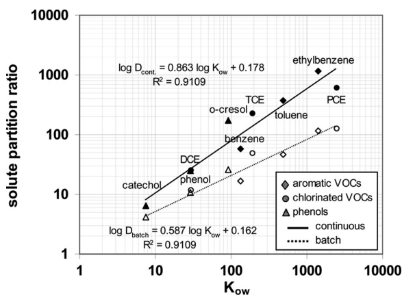
Figure 4. Comparisons of solute partition ratios in batch (open symbols) and continuous (closed symbols) operation as a function of octanol-water partition coefficient ( K_{ow} ) of the various solutes.
