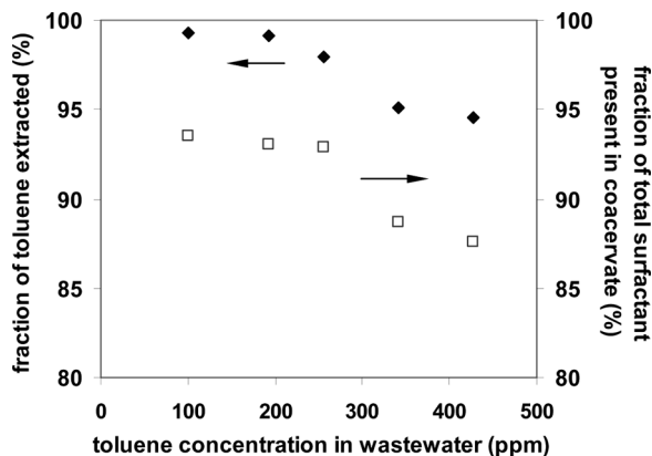
Figure 7. Fraction of toluene extracted and fraction of total surfactant present in coacervate as a function of toluene concentration in wastewater in continuous operation.
