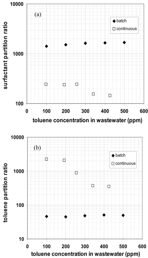
Figure 9 (a) and (b). Surfactant and toluene partition ratios of batch and continuous operation as a function of toluene concentration in wastewater respectively.
