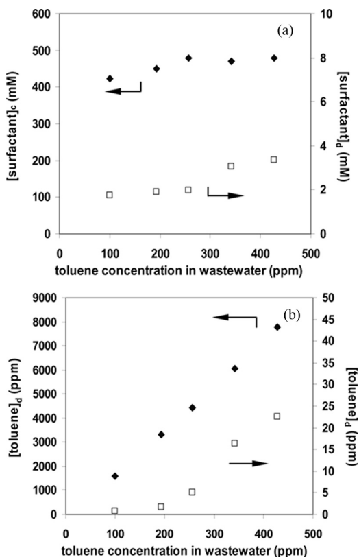
Figure 6 (a) and (b). Surfactant (a) and toluene (b) concentration in coacervate (c) and dilute phase (d) as a function of toluene concentration in wastewater in continuous operation, respectively.
